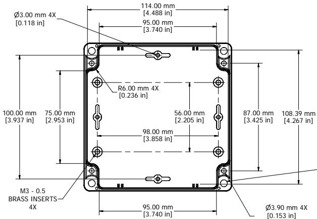
BOX - INSIDE
